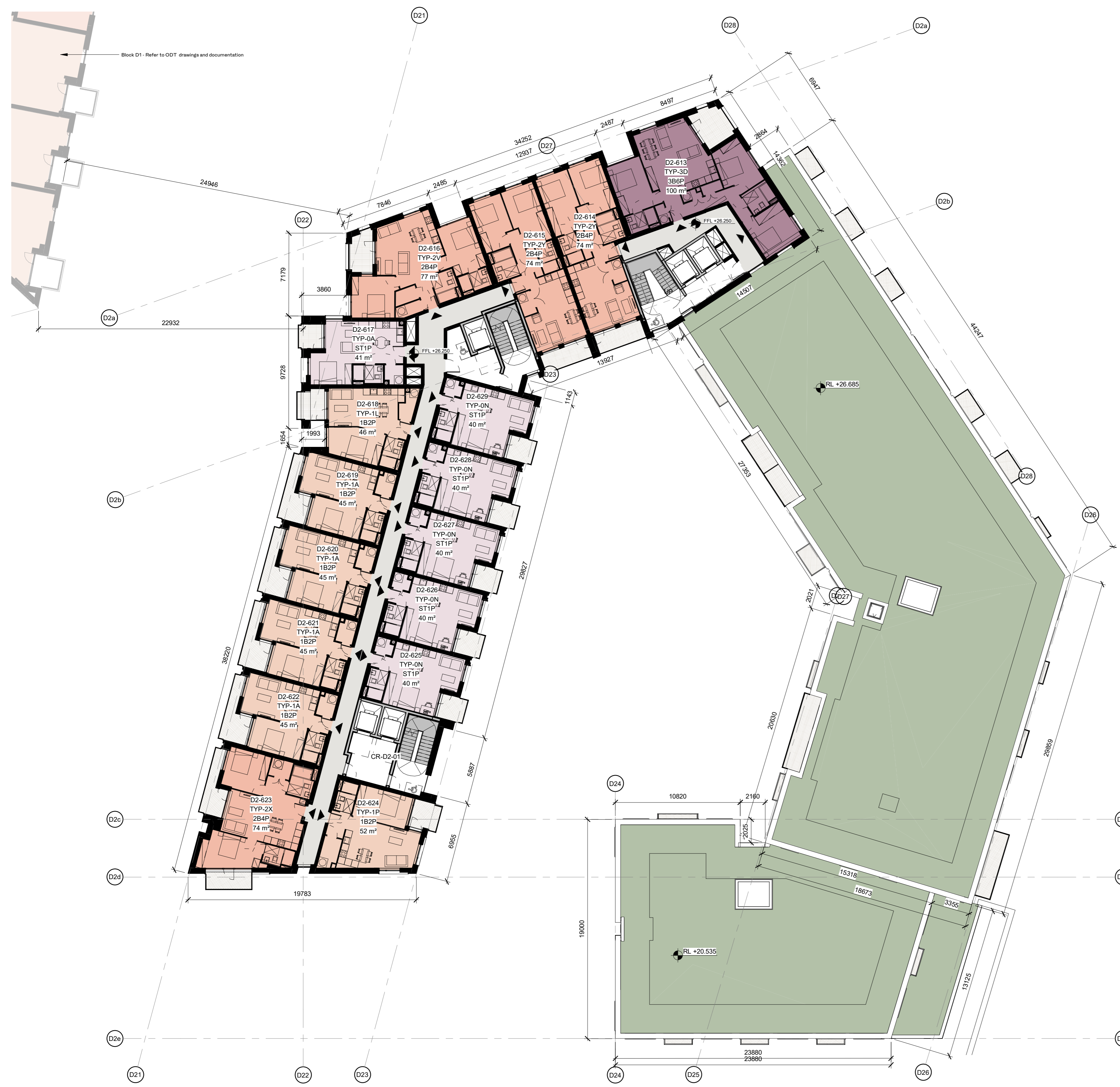
1 BLOCK D2-LEVEL 06 1 : 200
